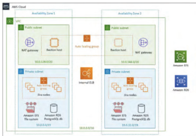
Architecture Diagram
